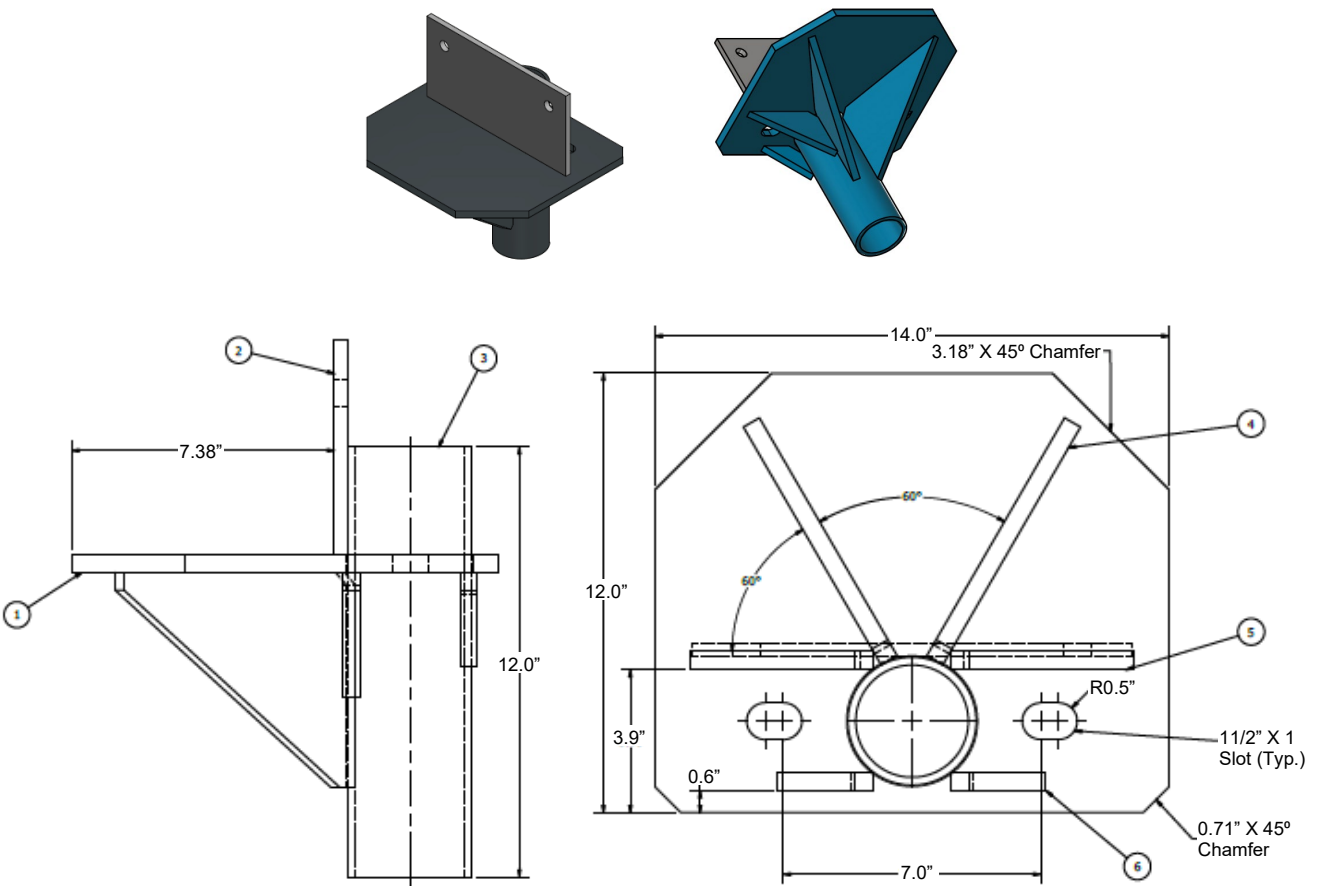
FIGURE 4—102 REPAIR BRACKET WITH BACK PLATE (Model No. FBB14121235)
