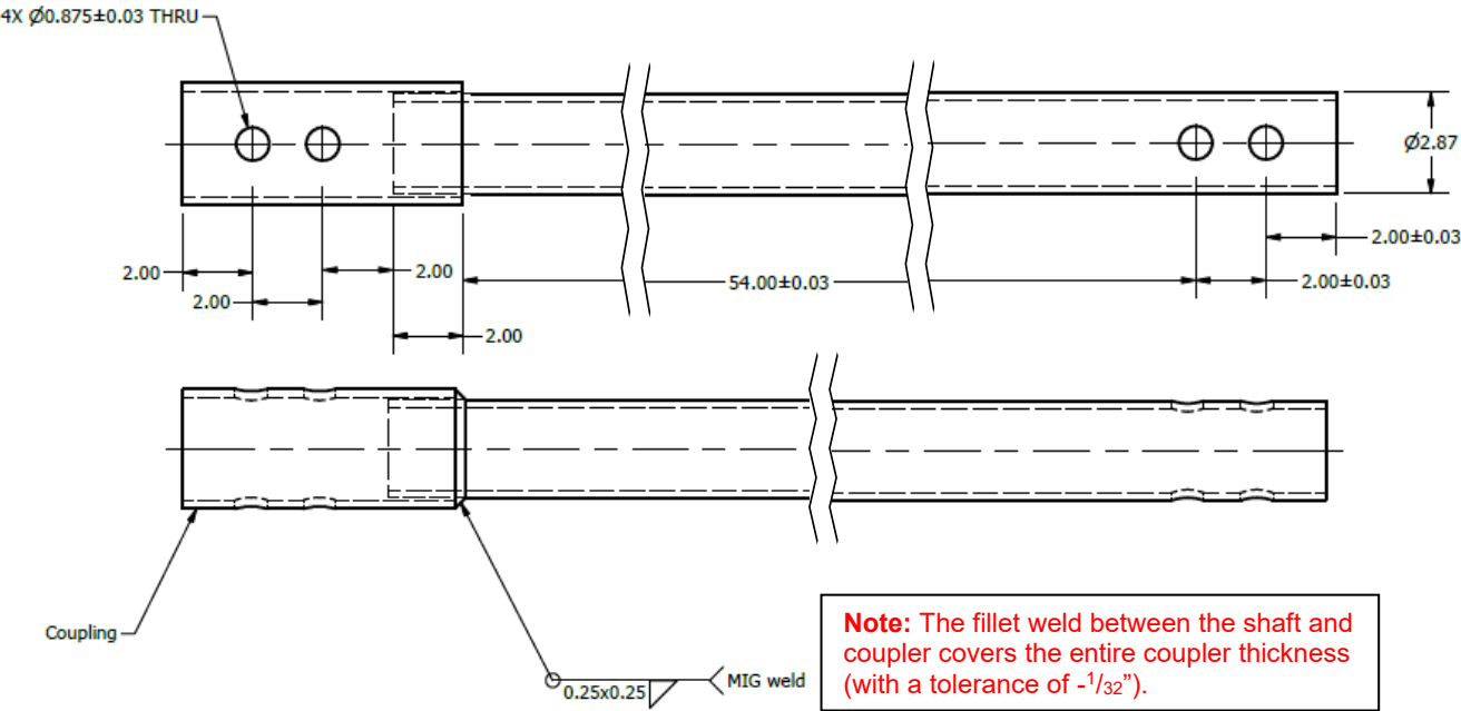
FIGURE 2—EXTENSION SHAFT SECTION OF THE 2 7 / 8 X 0.217-INCH HELICAL PILE (Model No. EXT2882175)
