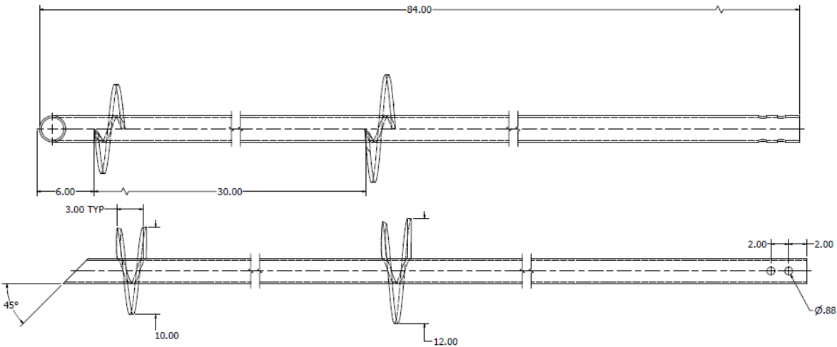
Model No. PP2870-702: Double Helix (10" & 12" Diameters) Lead Section
