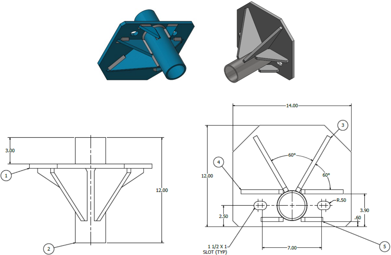
FIGURE 3—101 REPAIR BRACKET WITHOUT BACK PLATE (Model No. FB141212350)
