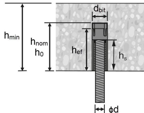
FIGURE 2—HILTI HDI-TZ INSTALLATION PARAMETERS IN CONCRETE
