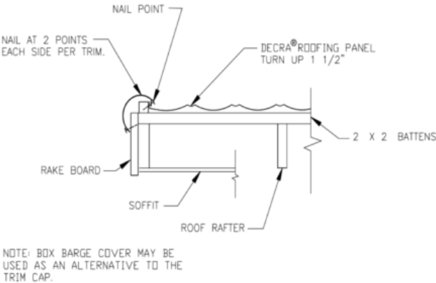
RAKE DETAIL WITH PANEL TURN UP
